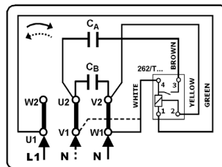
Figure 18 Single phase motor type 3SSIE with Start capacitor CA, run capacitor CB and centrifugal switch.
