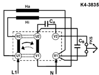
Figure 17 Single phase motor type SEMh-F with Start capacitor CA, run capacitor CB and centrifugal switch.
