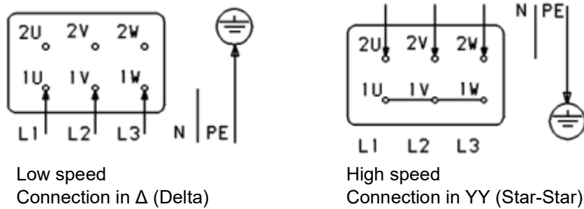
Figure 12 Three phase dual speed motor with single winding (Dahlander), like 4/2-, 8/4-, 12/6-pole
